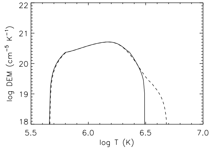
FIG. 8.—Coronal differential emission measure distribution for example 1 ( dashed curve ) and for a corresponding simulation in which half of the nanoflare energy takes the form of a nonthermal electron beam ( solid curve ).
